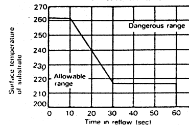
Reflow Method
